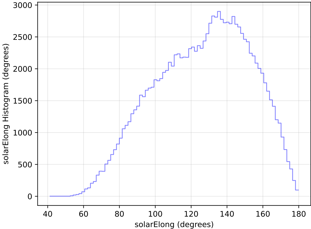
too_elab_r64_d2_ugrizy_v3.4_10yrs WFD u band: solarElong Histogram
