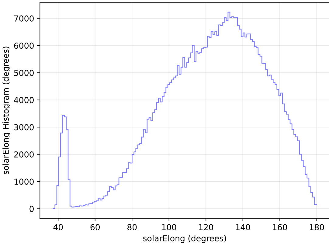
too_elab_r64_d2_ugrizy_v3.4_10yrs WFD r band: solarElong Histogram
