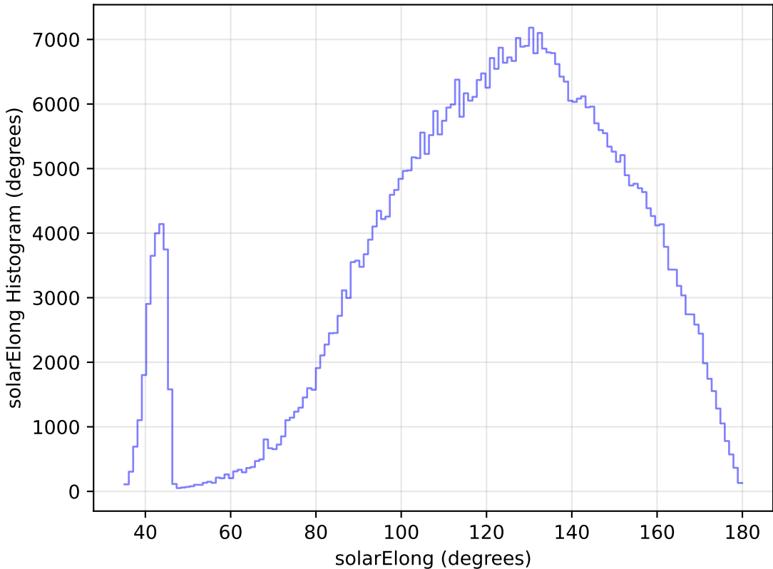
too_elab_r64_d2_ugrizy_v3.4_10yrs WFD i band: solarElong Histogram
