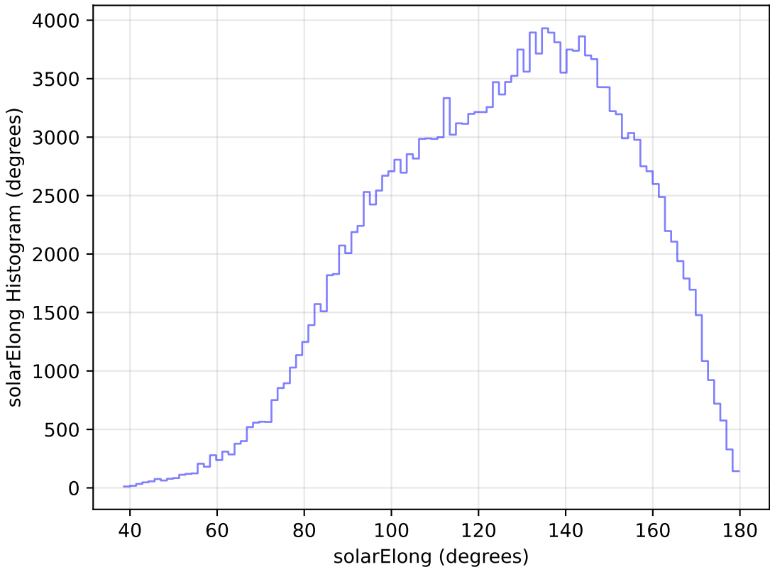
too_elab_r64_d2_ugrizy_v3.4_10yrs WFD g band: solarElong Histogram
