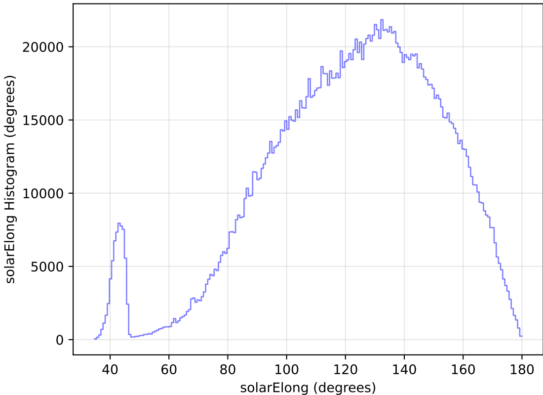
too_elab_r64_d2_ugrizy_v3.4_10yrs WFD all bands: solarElong Histogram
