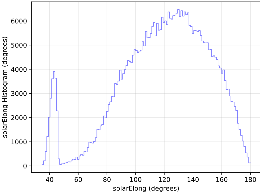
too_elab_r64_d2_ugrizy_v3.4_10yrs All sky z band: solarElong Histogram
