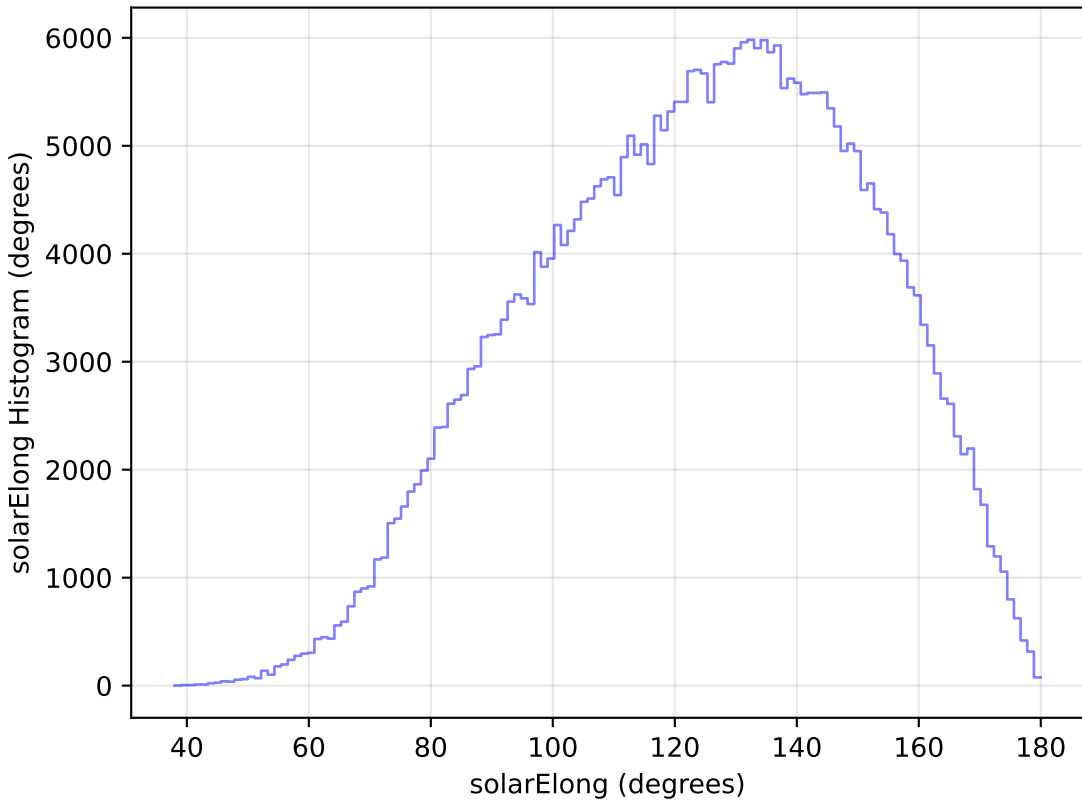
too_elab_r64_d2_ugrizy_v3.4_10yrs All sky y band: solarElong Histogram
