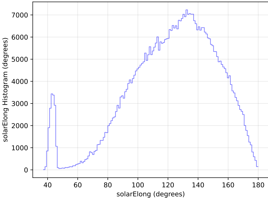
too_elab_r64_d2_ugrizy_v3.4_10yrs All sky r band: solarElong Histogram
