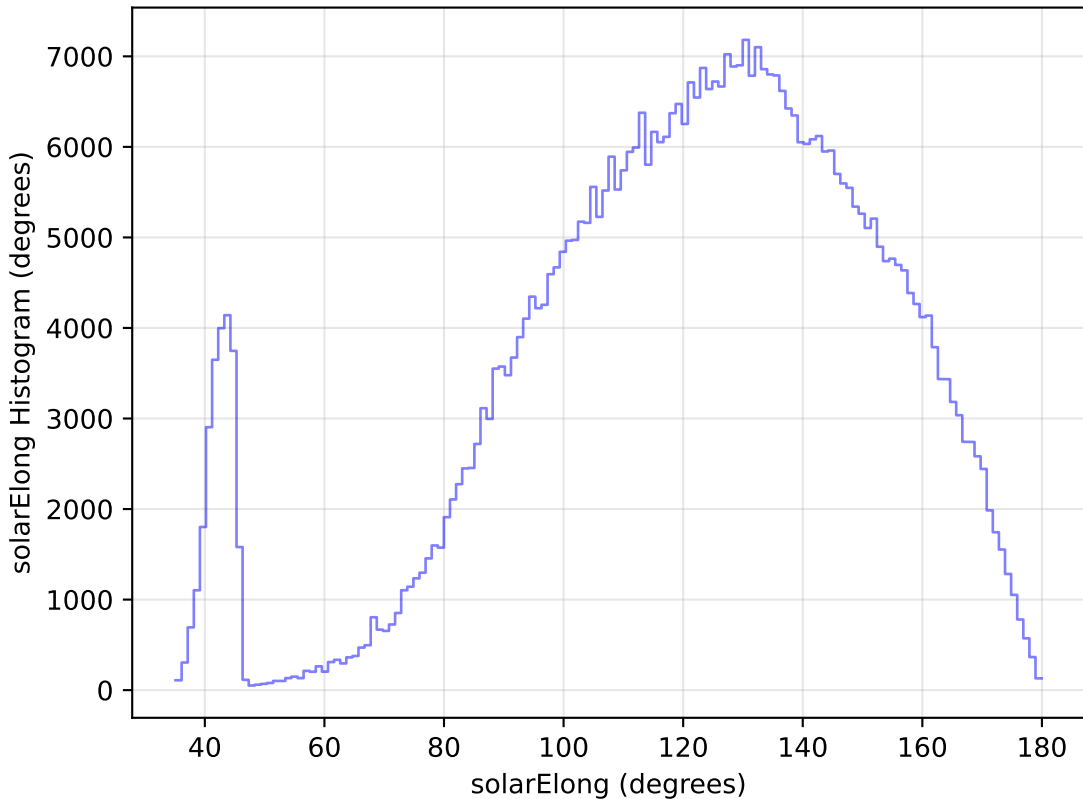
too_elab_r64_d2_ugrizy_v3.4_10yrs All sky i band: solarElong Histogram
