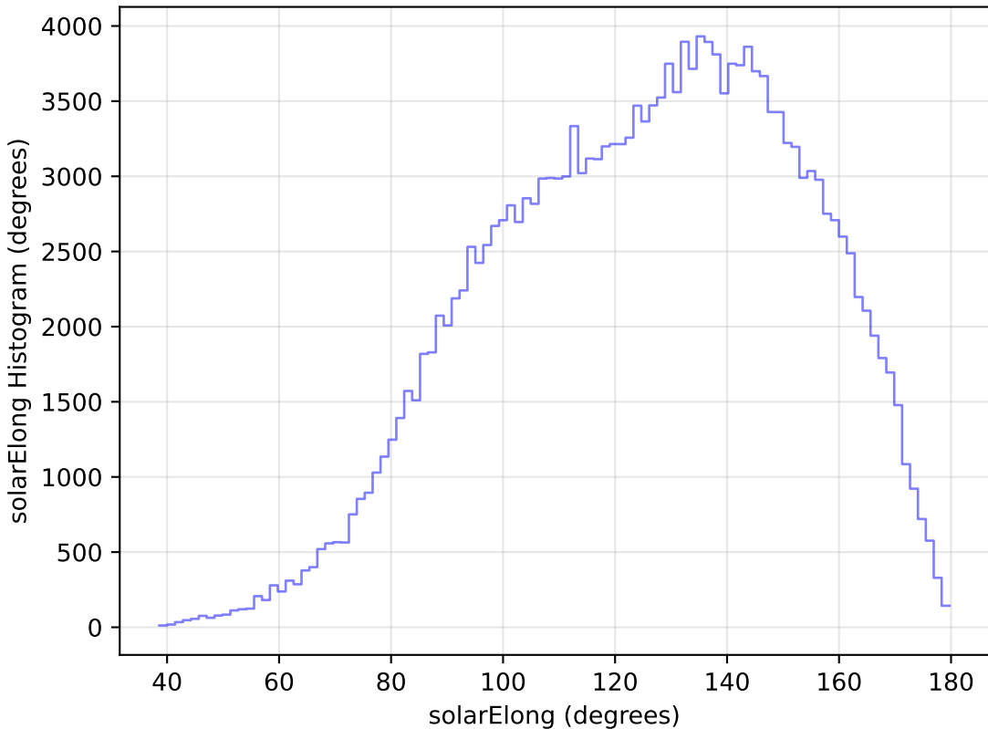
too_elab_r64_d2_ugrizy_v3.4_10yrs All sky g band: solarElong Histogram
