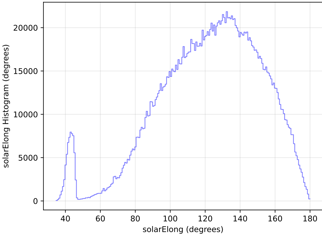
too_elab_r64_d2_ugrizy_v3.4_10yrs All sky all bands: solarElong Histogram
