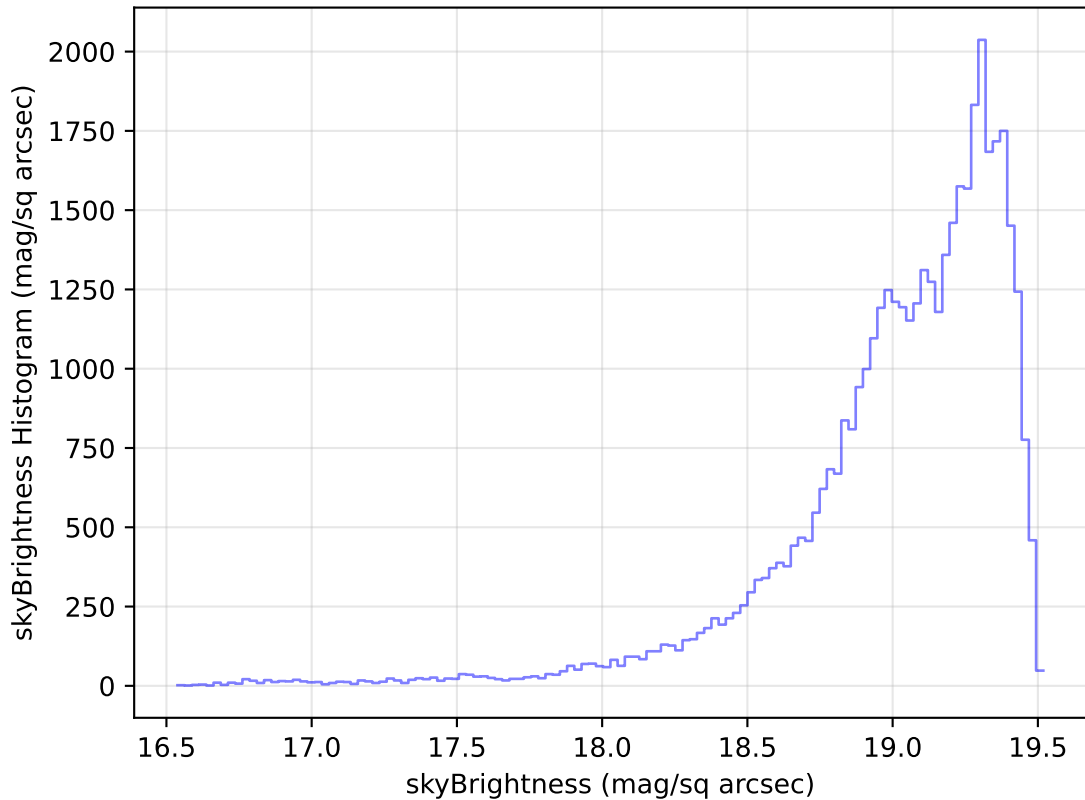
too_elab_r64_d2_ugrizy_v3.4_10yrs Yr 1 z band: skyBrightness Histogram
