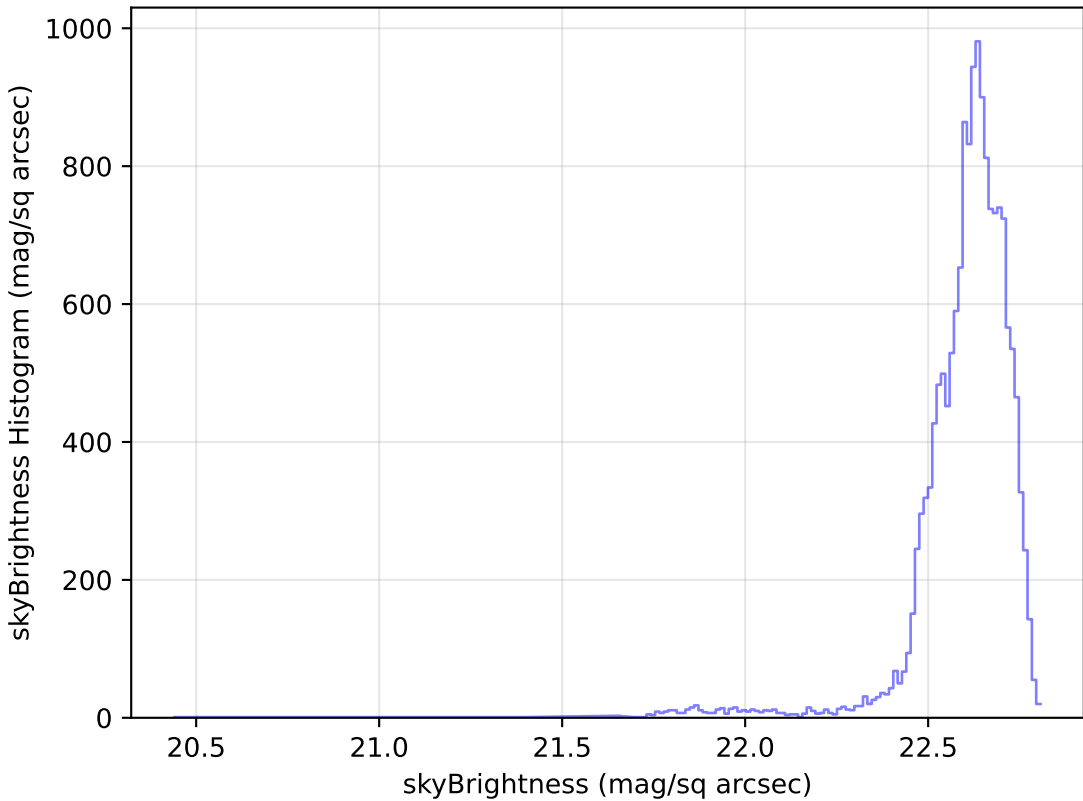
too_elab_r64_d2_ugrizy_v3.4_10yrs Yr 1 u band: skyBrightness Histogram
