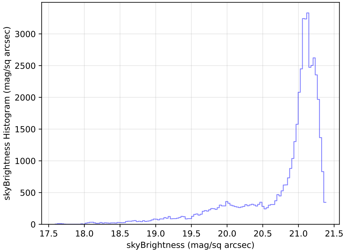
too_elab_r64_d2_ugrizy_v3.4_10yrs Yr 1 r band: skyBrightness Histogram
