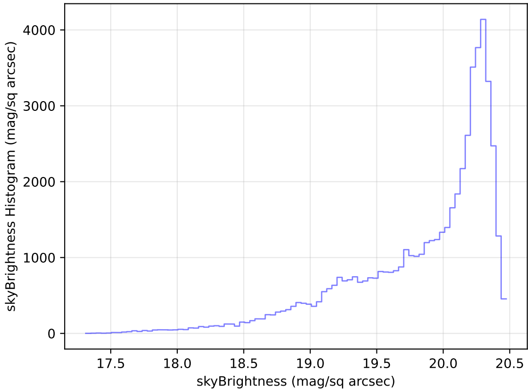
too_elab_r64_d2_ugrizy_v3.4_10yrs Yr 1 i band: skyBrightness Histogram
