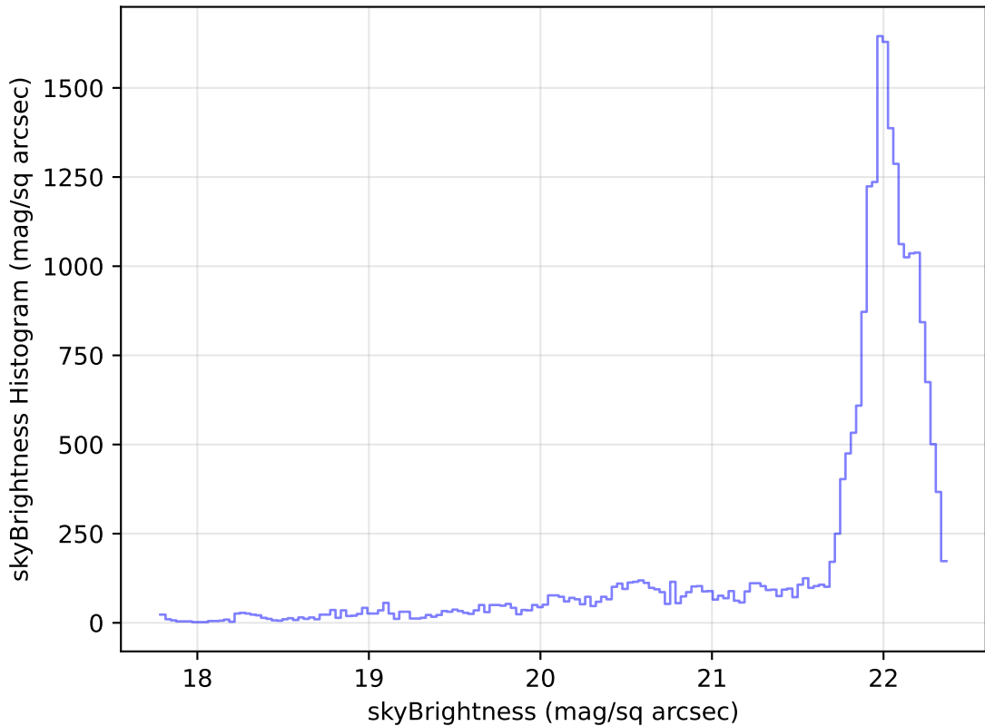
too_elab_r64_d2_ugrizy_v3.4_10yrs Yr 1 g band: skyBrightness Histogram
