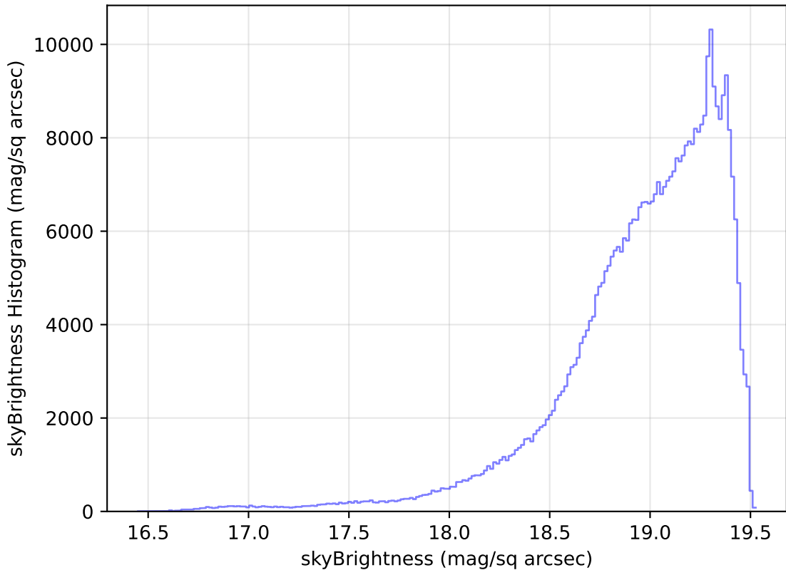
too_elab_r64_d2_ugrizy_v3.4_10yrs WFD z band: skyBrightness Histogram
