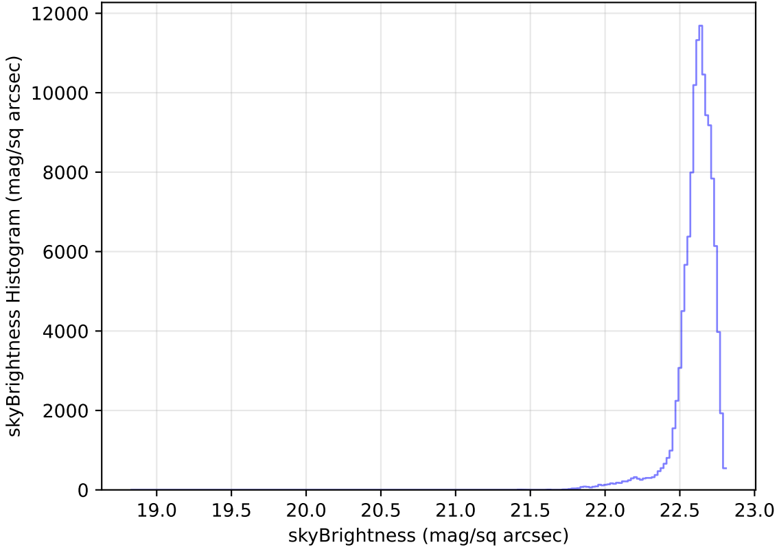
too_elab_r64_d2_ugrizy_v3.4_10yrs WFD u band: skyBrightness Histogram
