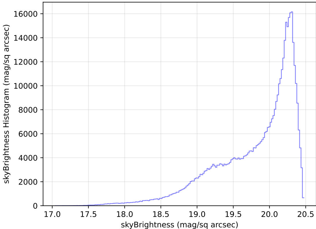
too_elab_r64_d2_ugrizy_v3.4_10yrs WFD i band: skyBrightness Histogram
