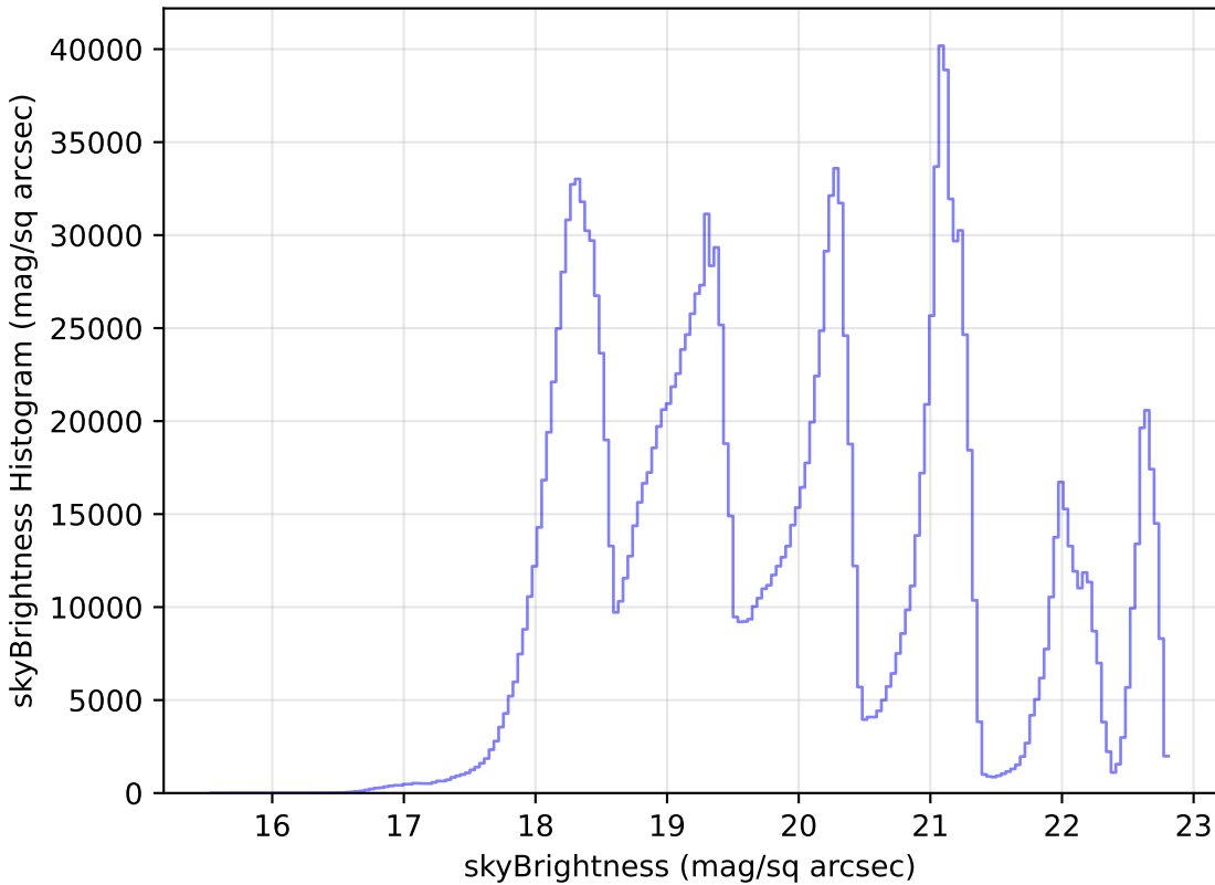
too_elab_r64_d2_ugrizy_v3.4_10yrs WFD all bands: skyBrightness Histogram
