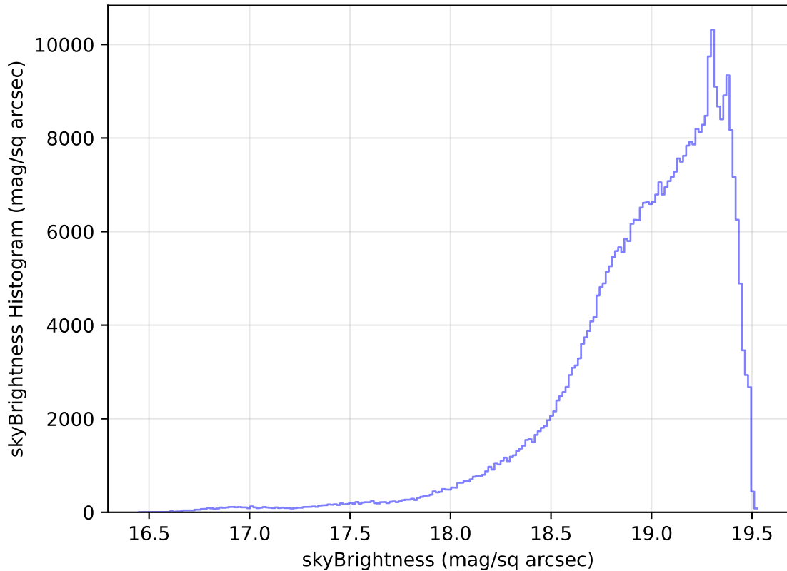
too_elab_r64_d2_ugrizy_v3.4_10yrs All sky z band: skyBrightness Histogram
