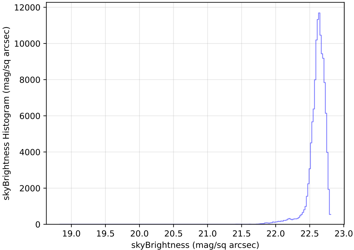
too_elab_r64_d2_ugrizy_v3.4_10yrs All sky u band: skyBrightness Histogram
