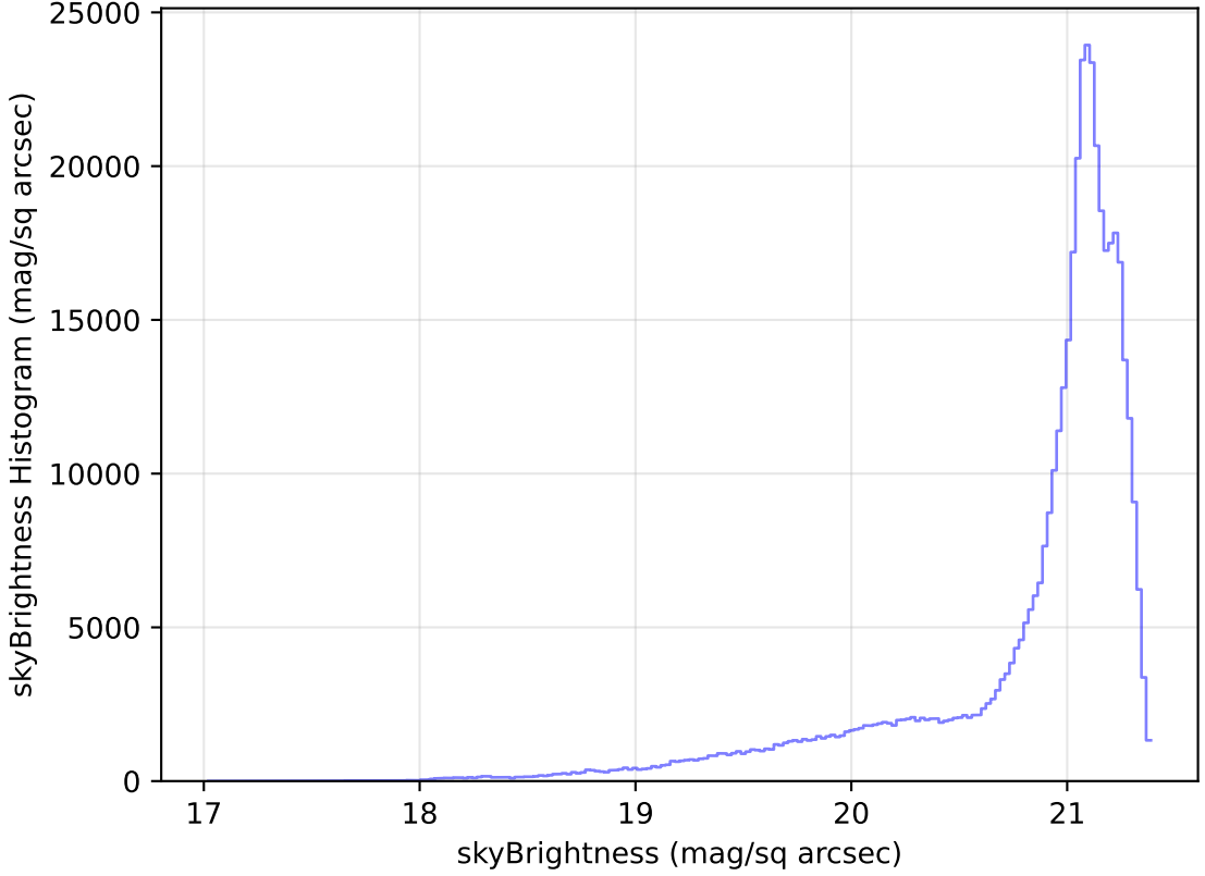
too_elab_r64_d2_ugrizy_v3.4_10yrs All sky r band: skyBrightness Histogram
