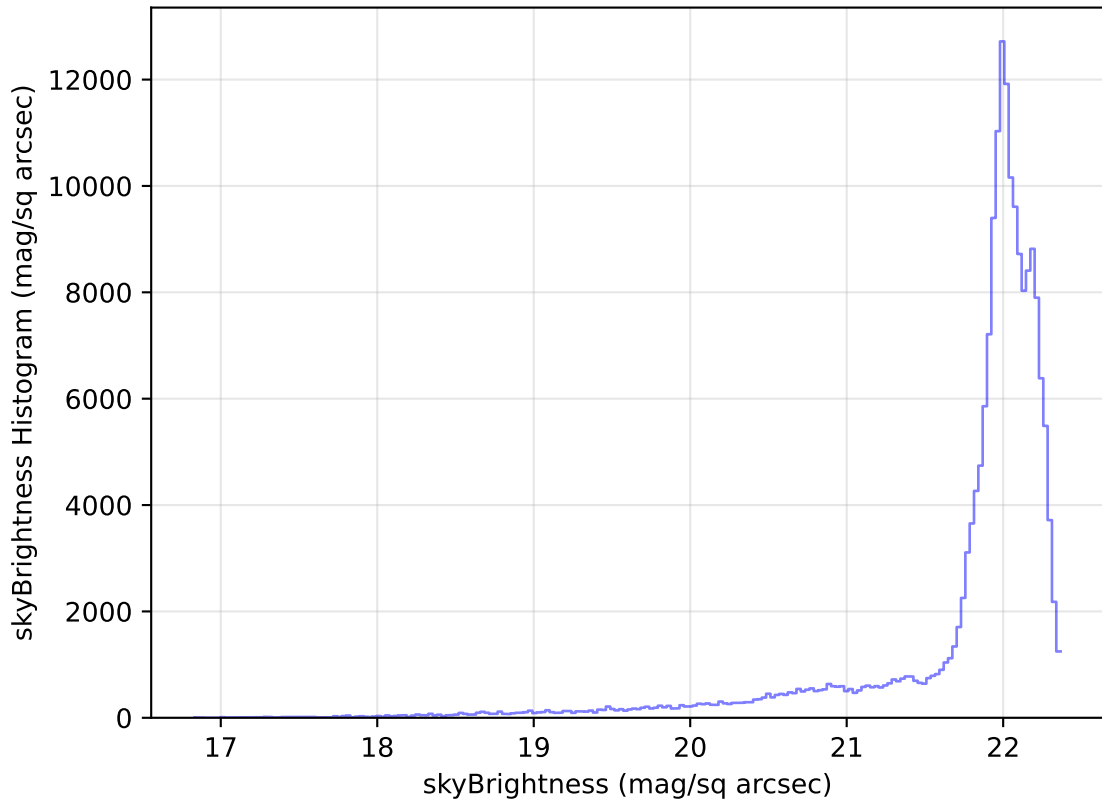
too_elab_r64_d2_ugrizy_v3.4_10yrs All sky g band: skyBrightness Histogram
