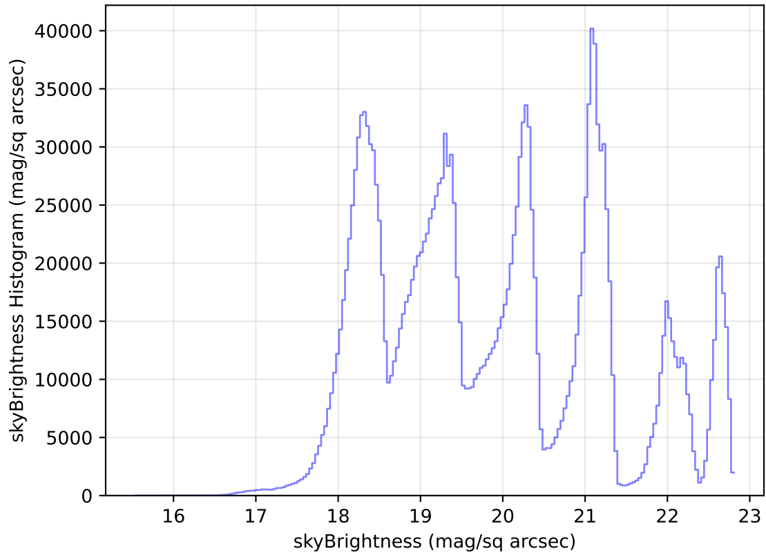
too_elab_r64_d2_ugrizy_v3.4_10yrs All sky all bands: skyBrightness Histogram
