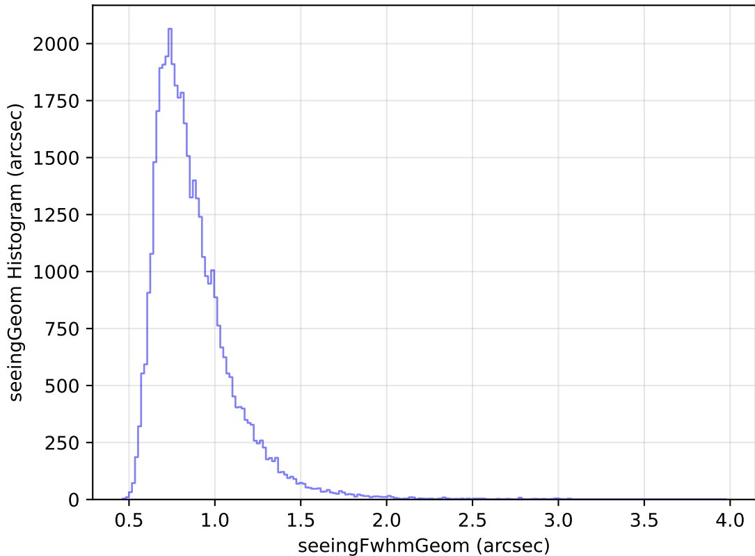
too_elab_r64_d2_ugrizy_v3.4_10yrs Yr 1 z band: seeingGeom Histogram
