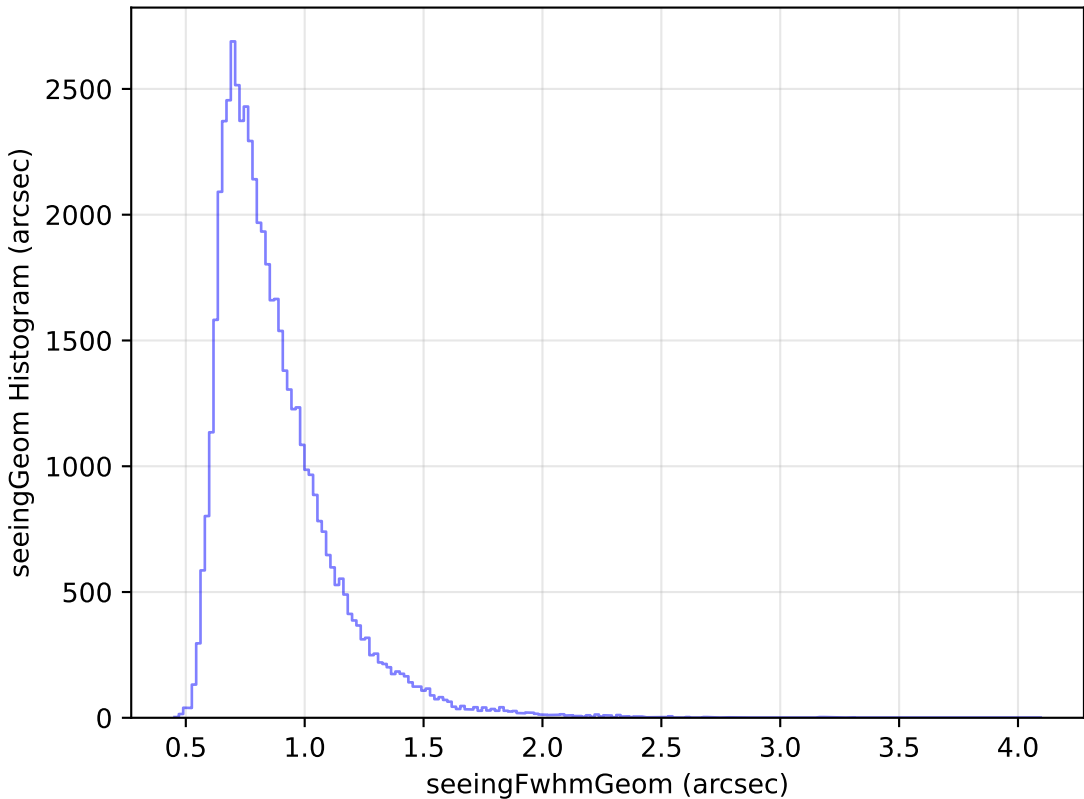
too_elab_r64_d2_ugrizy_v3.4_10yrs Yr 1 i band: seeingGeom Histogram
