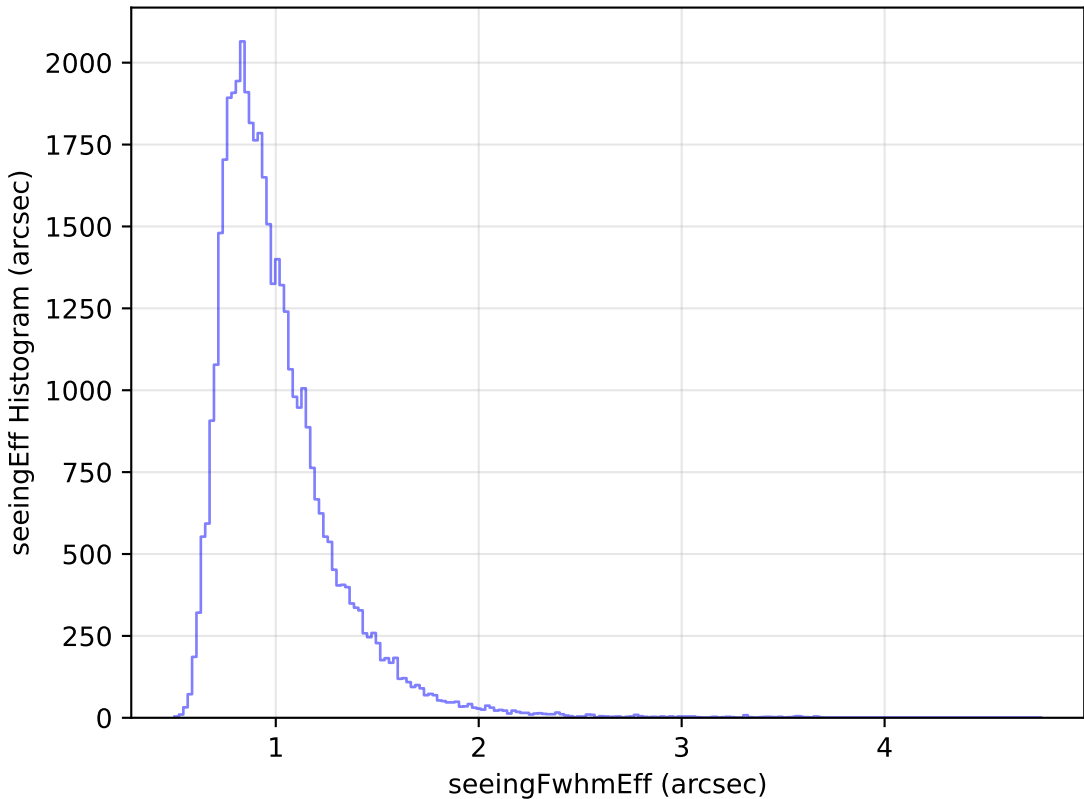
too_elab_r64_d2_ugrizy_v3.4_10yrs Yr 1 z band: seeingEff Histogram
