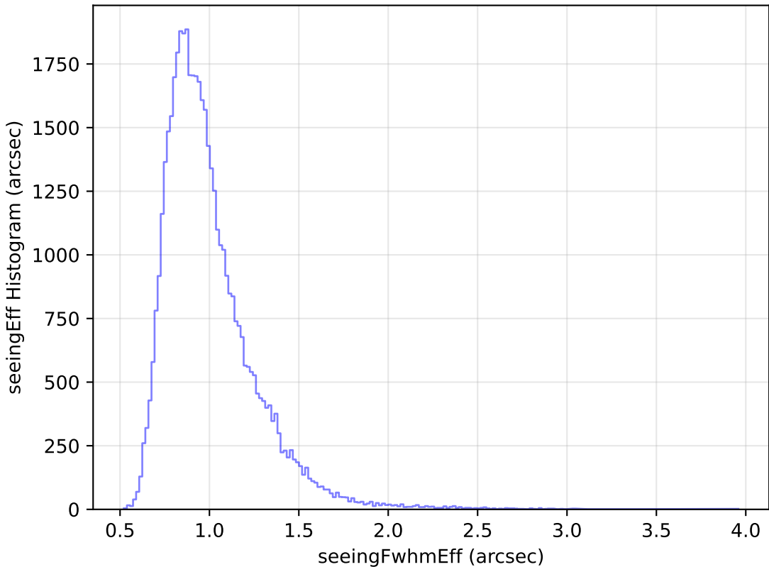
too_elab_r64_d2_ugrizy_v3.4_10yrs Yr 1 y band: seeingEff Histogram
