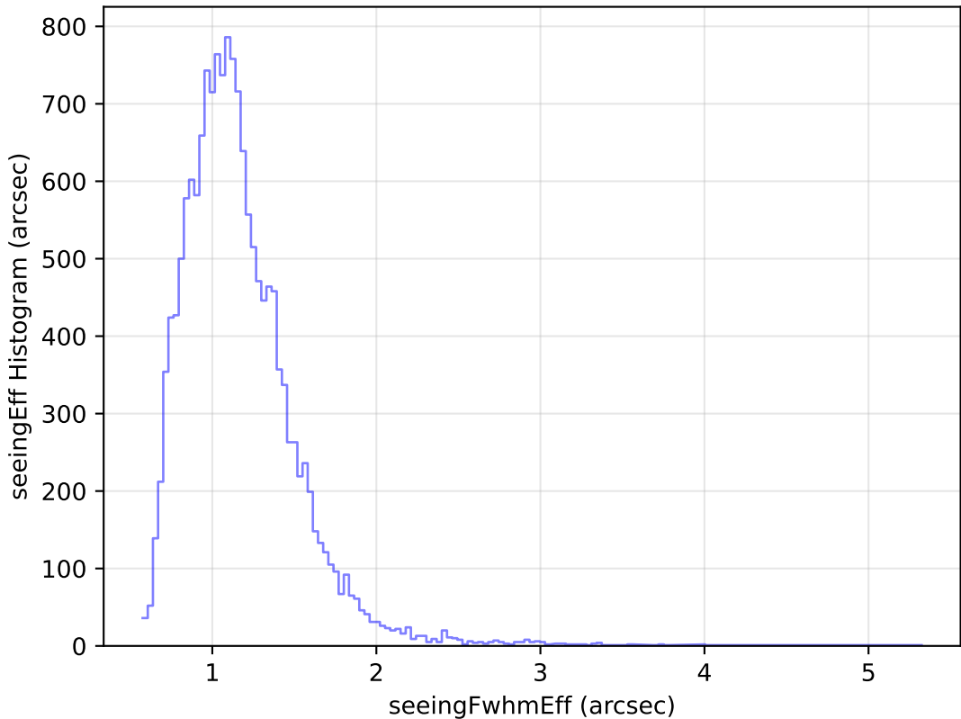
too_elab_r64_d2_ugrizy_v3.4_10yrs Yr 1 u band: seeingEff Histogram
