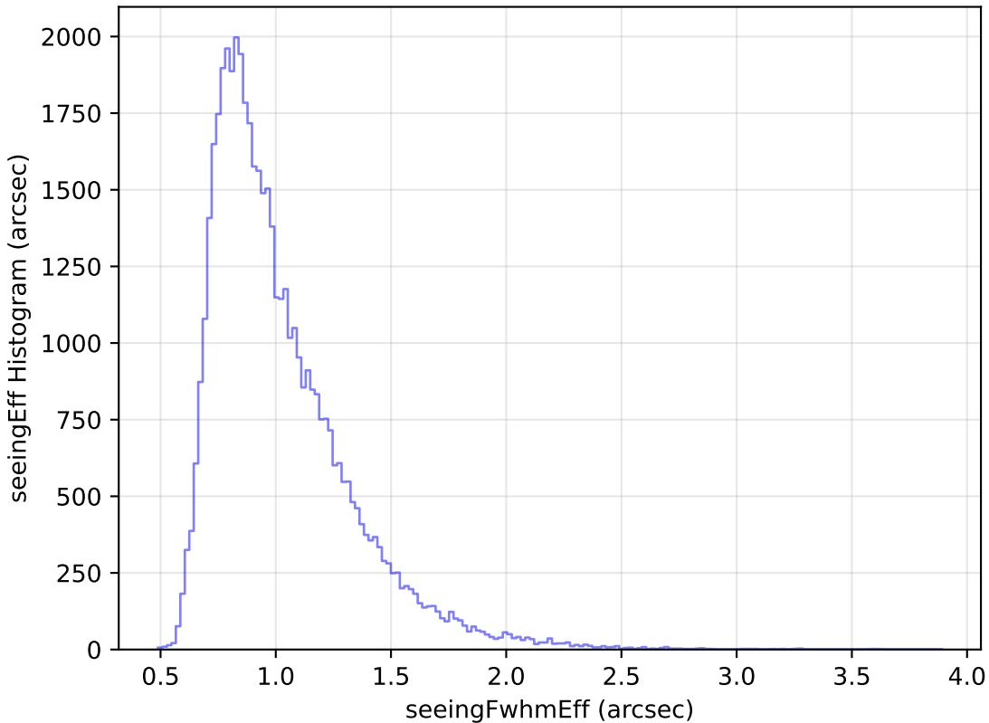
too_elab_r64_d2_ugrizy_v3.4_10yrs Yr 1 r band: seeingEff Histogram
