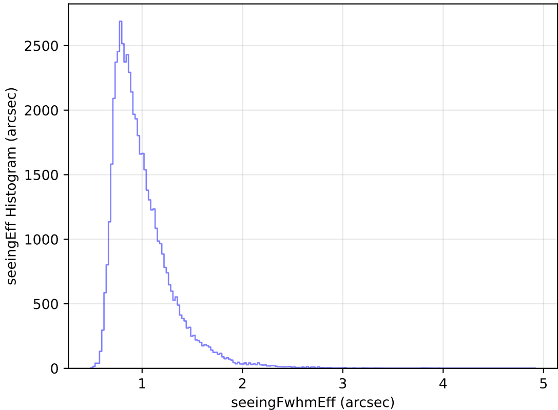
too_elab_r64_d2_ugrizy_v3.4_10yrs Yr 1 i band: seeingEff Histogram
