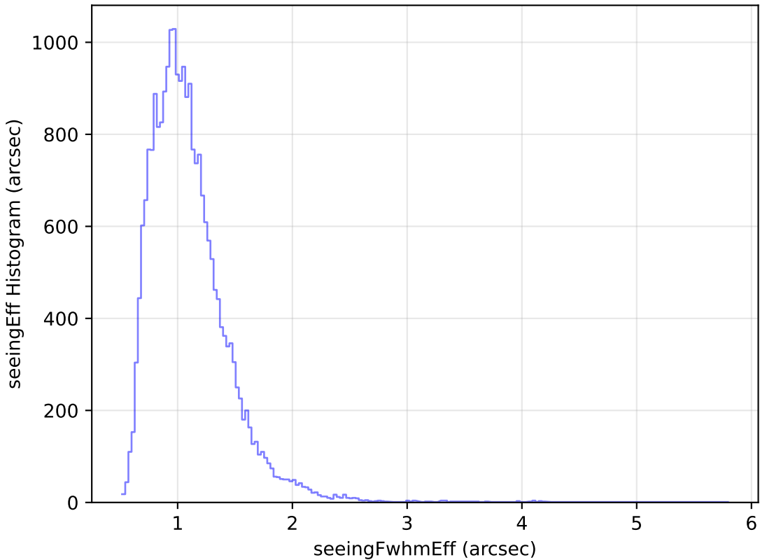
too_elab_r64_d2_ugrizy_v3.4_10yrs Yr 1 g band: seeingEff Histogram
