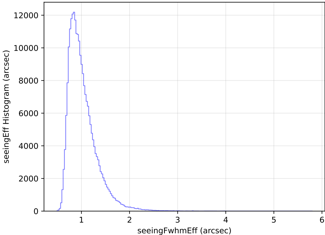
too_elab_r64_d2_ugrizy_v3.4_10yrs Yr 1 all bands: seeingEff Histogram
