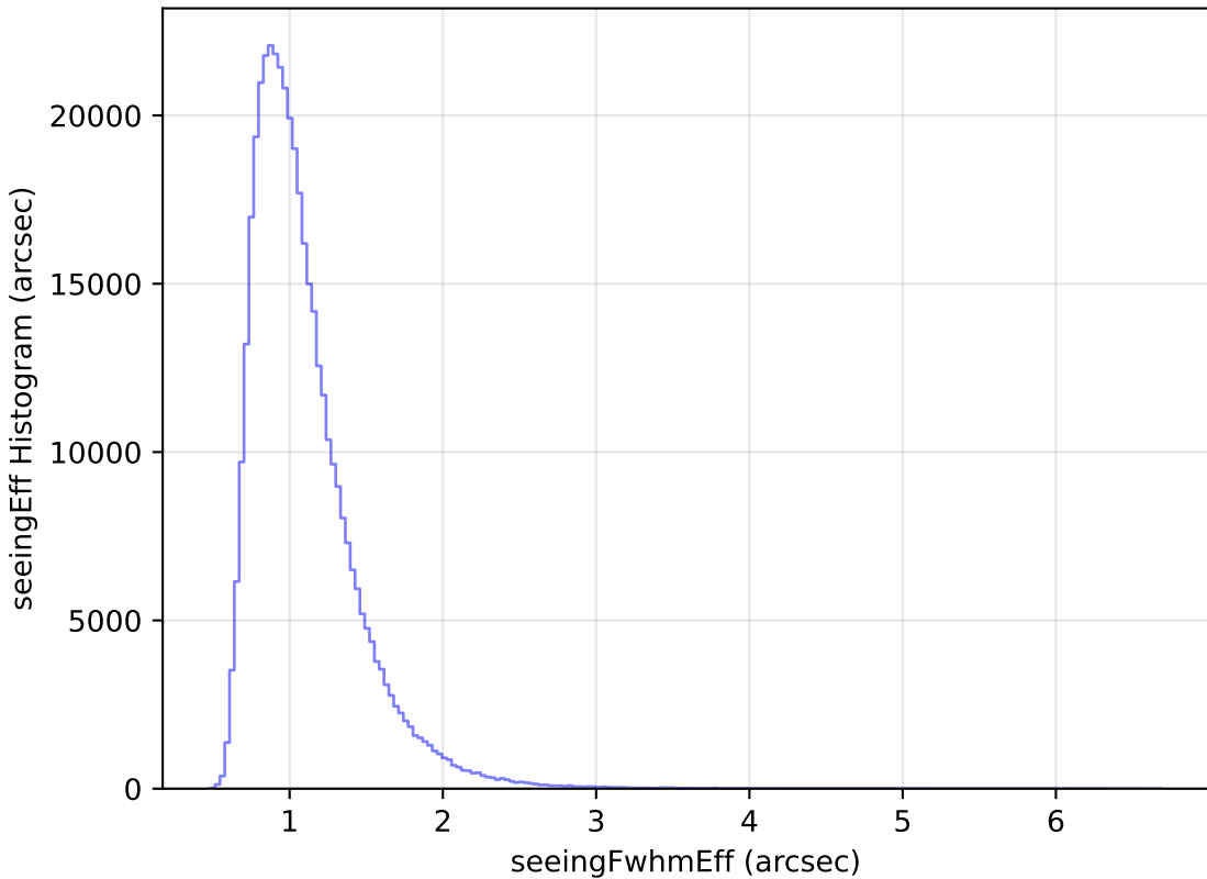
too_elab_r64_d2_ugrizy_v3.4_10yrs WFD z band: seeingEff Histogram
