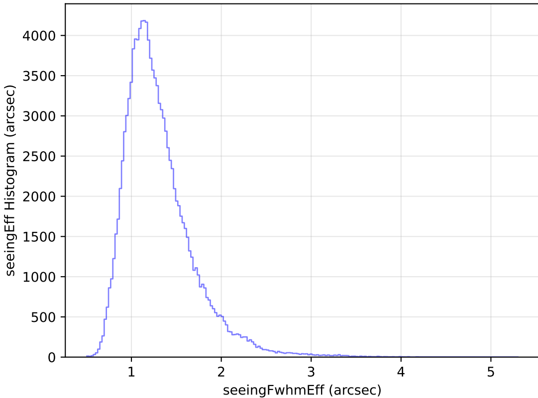
too_elab_r64_d2_ugrizy_v3.4_10yrs WFD u band: seeingEff Histogram
