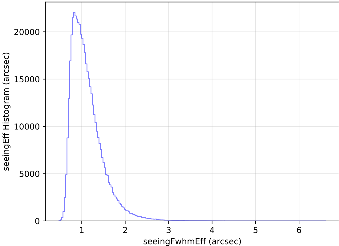
too_elab_r64_d2_ugrizy_v3.4_10yrs WFD r band: seeingEff Histogram
