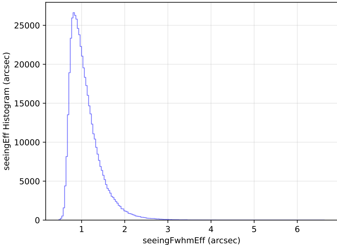
too_elab_r64_d2_ugrizy_v3.4_10yrs WFD i band: seeingEff Histogram
