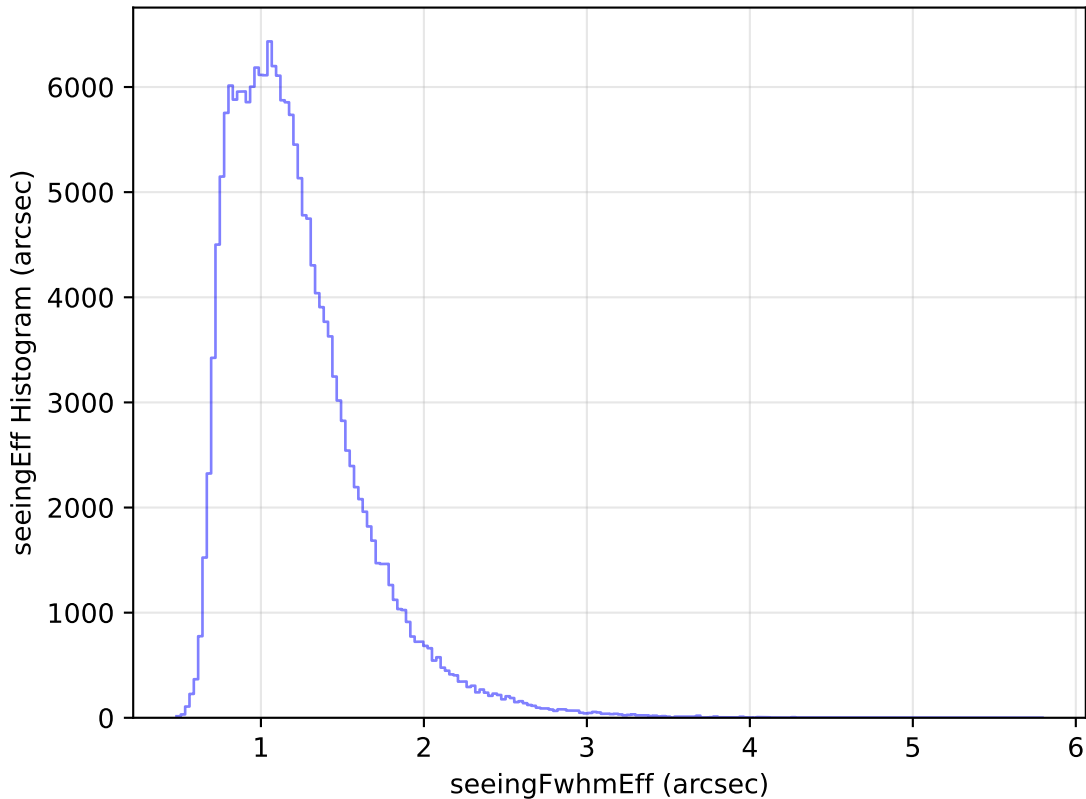
too_elab_r64_d2_ugrizy_v3.4_10yrs WFD g band: seeingEff Histogram
