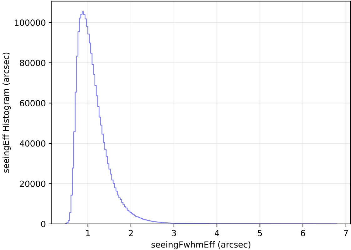
too_elab_r64_d2_ugrizy_v3.4_10yrs WFD all bands: seeingEff Histogram
