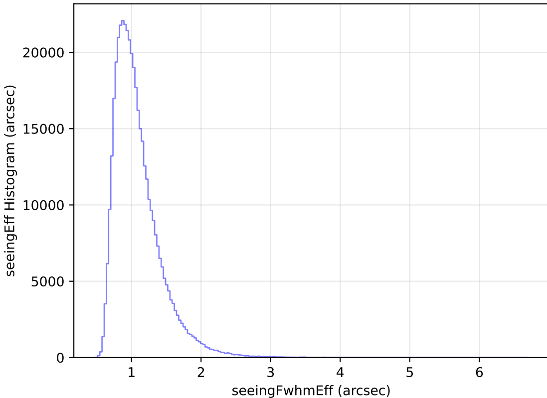
too_elab_r64_d2_ugrizy_v3.4_10yrs All sky z band: seeingEff Histogram
