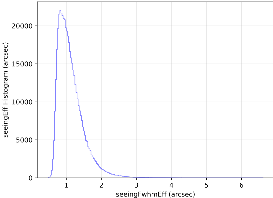
too_elab_r64_d2_ugrizy_v3.4_10yrs All sky r band: seeingEff Histogram
