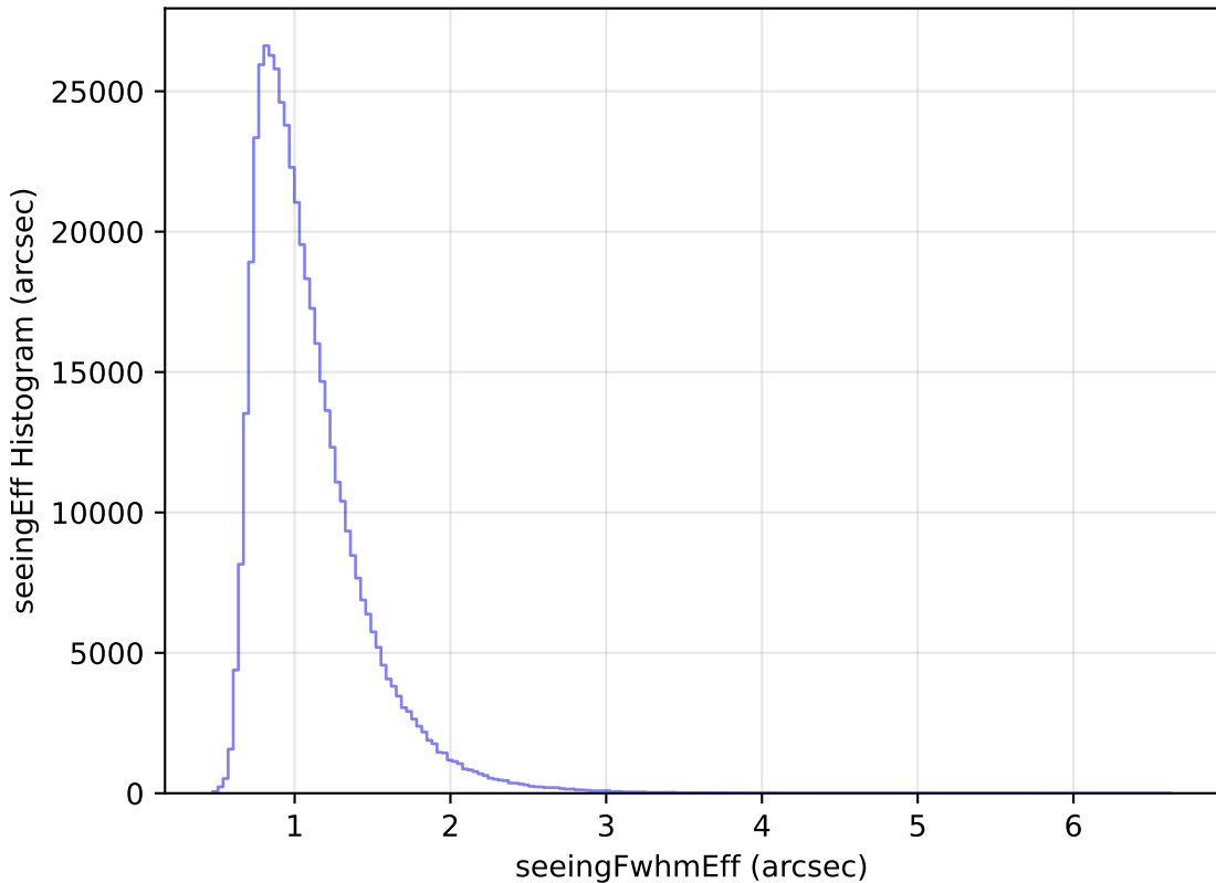
too_elab_r64_d2_ugrizy_v3.4_10yrs All sky i band: seeingEff Histogram
