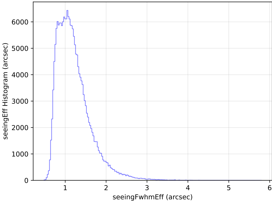
too_elab_r64_d2_ugrizy_v3.4_10yrs All sky g band: seeingEff Histogram
