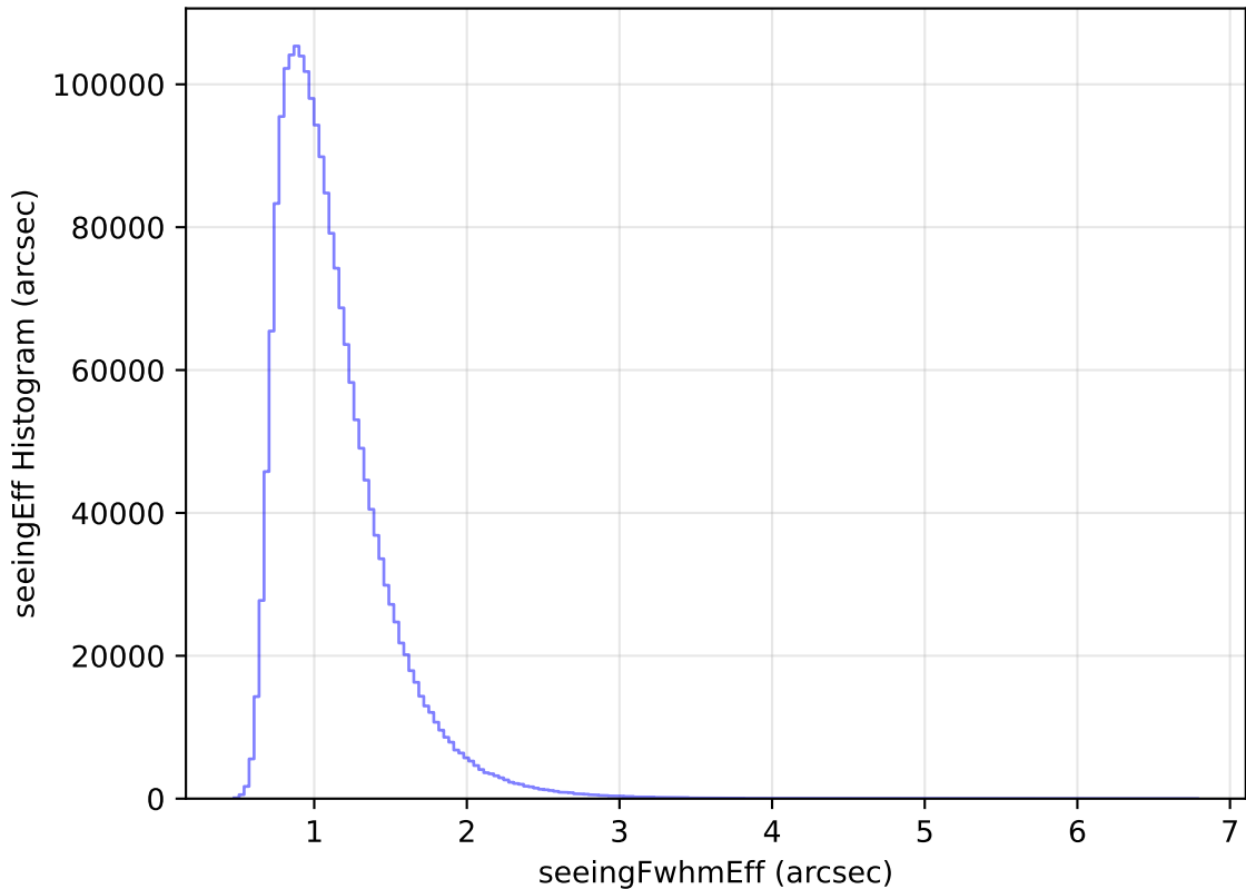
too_elab_r64_d2_ugrizy_v3.4_10yrs All sky all bands: seeingEff Histogram
