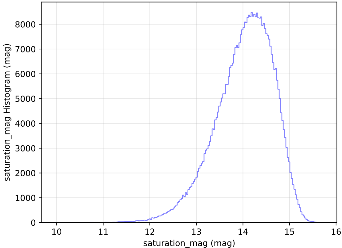
too_elab_r64_d2_ugrizy_v3.4_10yrs_WFD_z_band: saturation_mag Histogram
