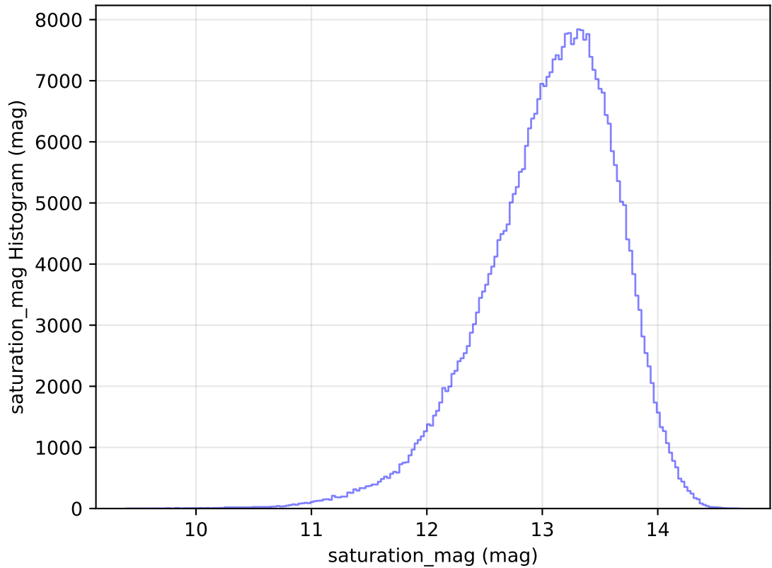
too_elab_r64_d2_ugrizy_v3.4_10yrs WFD y band: saturation_mag Histogram
