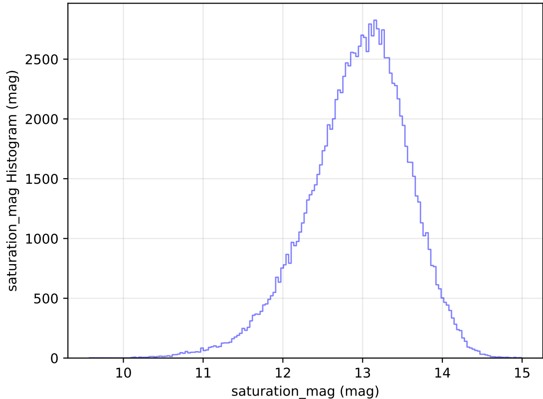
too_elab_r64_d2_ugrizy_v3.4_10yrs WFD u band: saturation_mag Histogram
