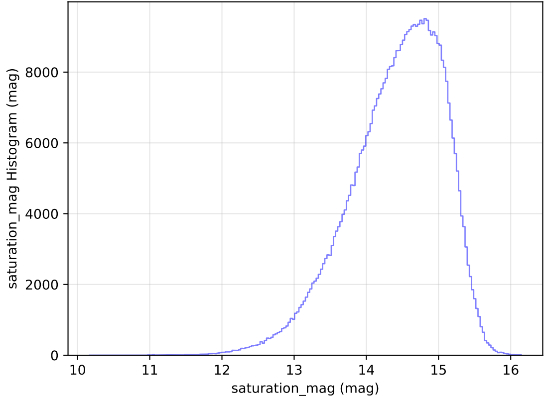
too_elab_r64_d2_ugrizy_v3.4_10yrs WFD i band: saturation_mag Histogram
