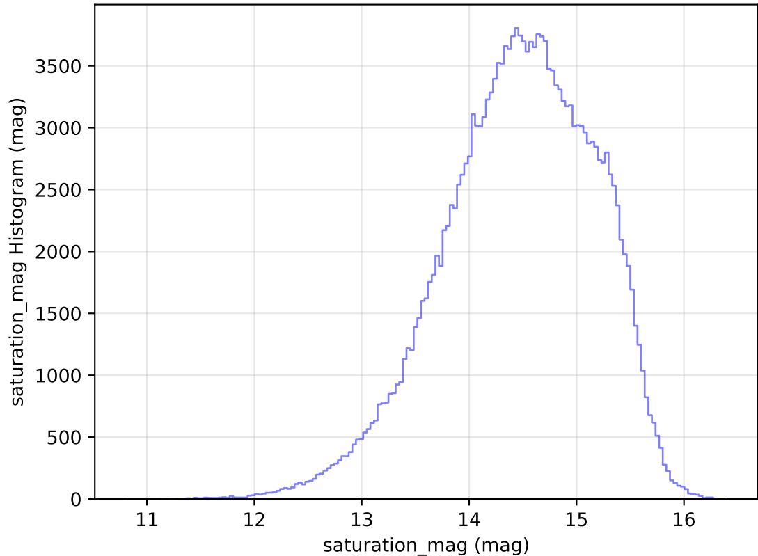
too_elab_r64_d2_ugrizy_v3.4_10yrs WFD g band: saturation_mag Histogram
